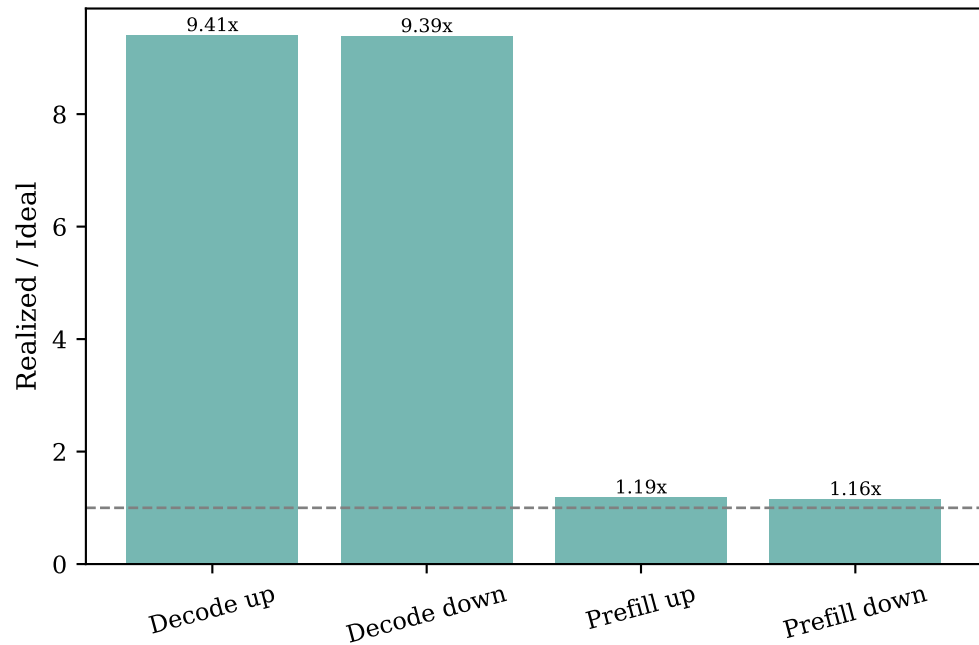
W4A4 Latency Gap vs Ideal
