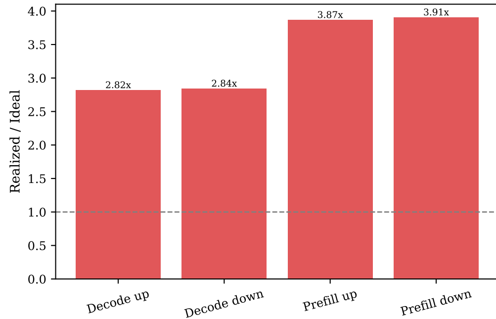
W4A4 Energy Gap vs Ideal
